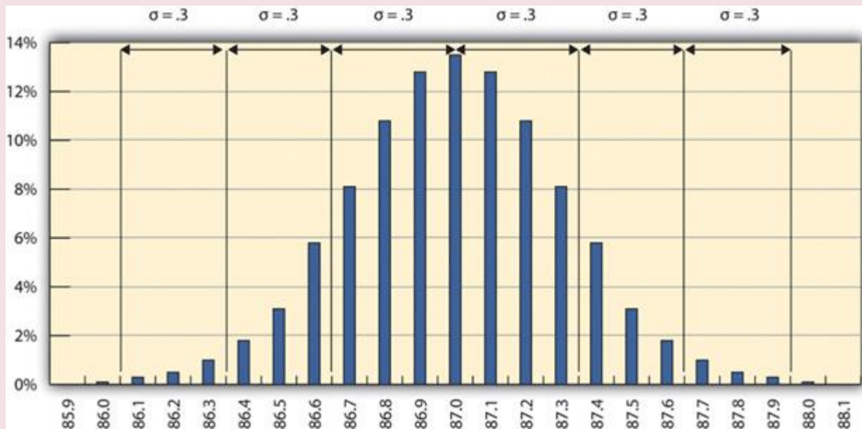
Figure 14.3 The 68-95-99.7 Rule
