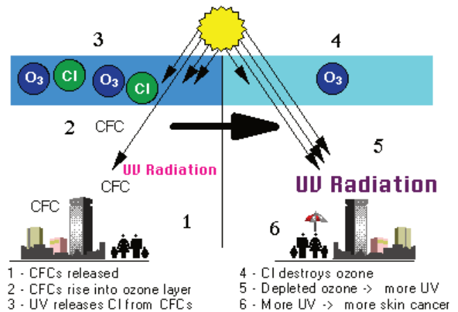
Figure 1. Strong UV light breaks apart the ODS molecule. CFCs, HCFCs, carbon tetrachloride, methyl chloroform, and other gases release chlorine atoms, and halons and methyl bromide release bromine atoms. It is these atoms that actually destroy ozone, not the intact ODS molecule. It is estimated that one chlorine atom can destroy over 100,000 ozone molecules before it is removed from the stratosphere. Credit: NASA GSFC.
