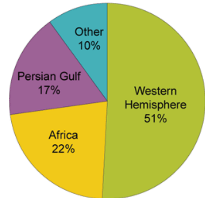
Figure 2. Sources of United States Net Petroleum Imports, 2009 Figure illustrates that the United States imported over half of the crude oil and refined petroleum products that it consumed during 2009. Source: U.S. Energy Information Administration, Petroleum Supply Annual, 2009 , preliminary data.
