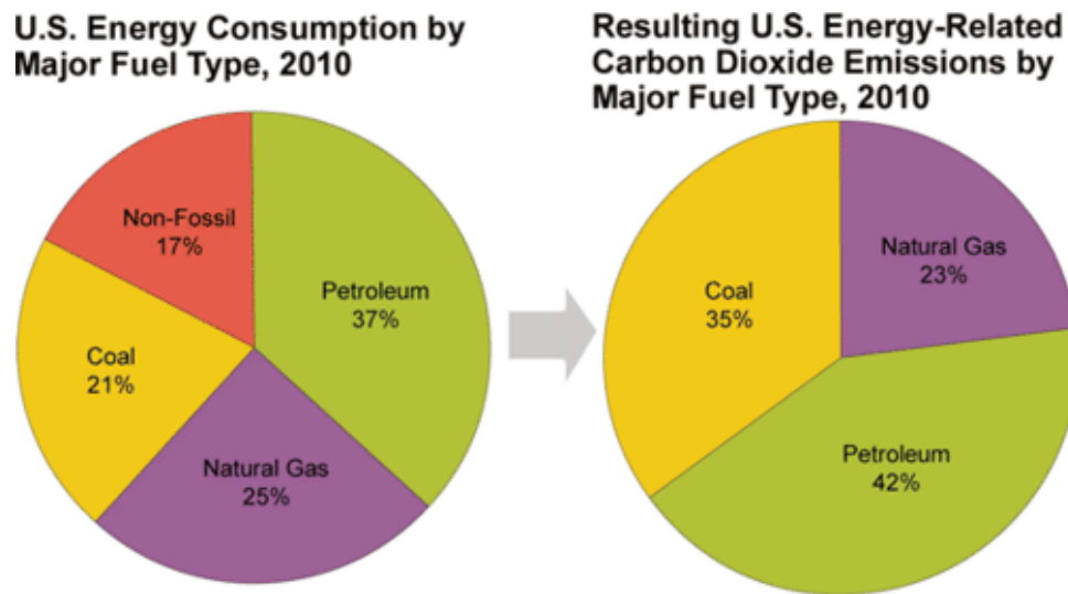
Figure 4. Fuel Type and Carbon Emissions The two charts show the relationship between fuel type and carbon emissions for U.S. energy consumption in 2010. Source: U.S. Energy Information Administration
