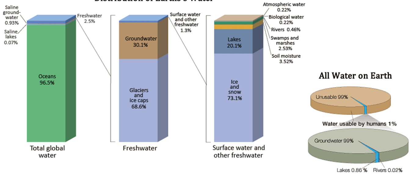
Figure 1. Earth's Water Reservoirs. Bar chart Distribution of Earth's water including total global water, fresh water, and surface water and other fresh water and Pie chart Water usable by humans and sources of usable water. Source: United States Geographical Survey Igor Skiklomanov's chapter "World fresh water resources" in Peter H. Gleick (editor), 1993, Water in Crisis: A Guide to the World's Fresh Water Resources
