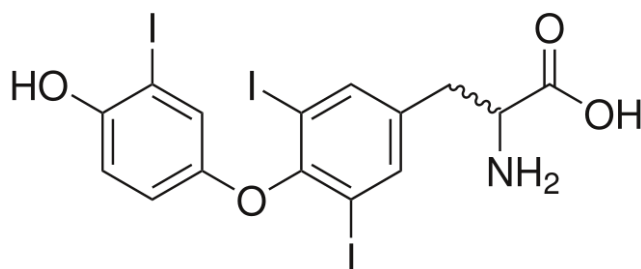
Figure 10.111 The structure of triiodothyronine ( T_3 ) 1
