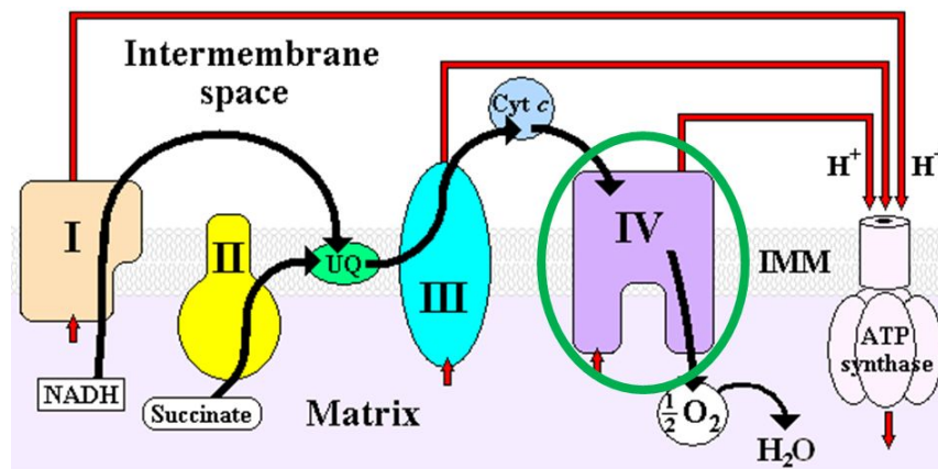
Figure 12.915 Cytochrome c oxidase (complex IV) 3
