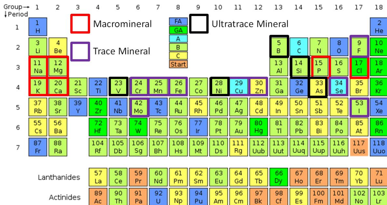
Figure 8.21 Minerals are a subset of elements, this figure shows their position within the periodic table 2
