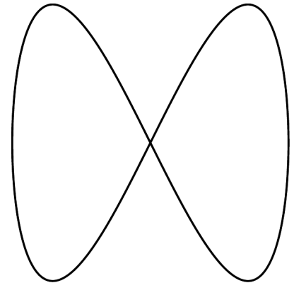
a / The Lissajous figure x = \cos t , y = \sin 2t .
