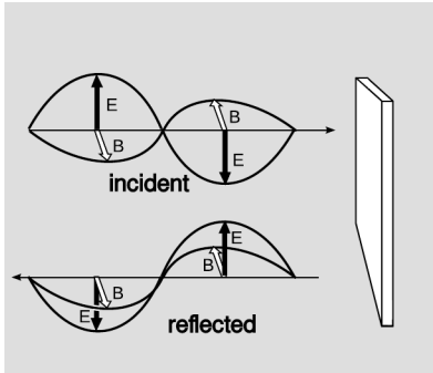
j / Example 23. The incident and reflected waves are drawn offset from each other for clarity, but are actually on top of each other so that their fields superpose.
