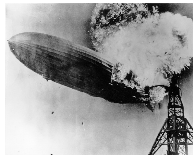
m / Hydrogen is highly reactive.
