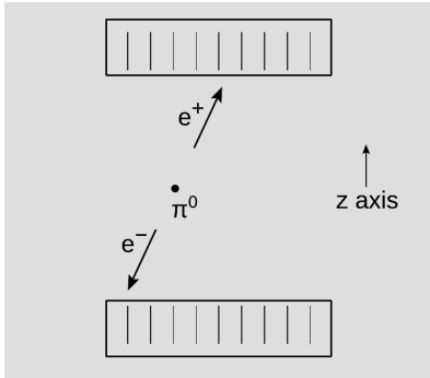
b / The decay of a neutral pion is detected through its decay products.
