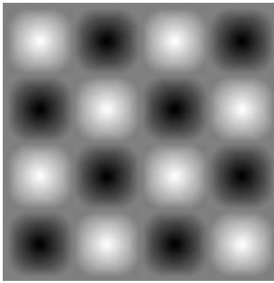
c / A solution to the Schrödinger equation found by separability. Positive values are shown as light colors, negative ones as dark colors.
