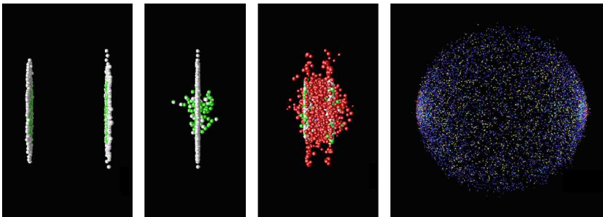
r / Colliding nuclei show relativistic length contraction.
