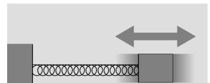
d / The time for one cycle of vibration is related to the object's inertial mass.
