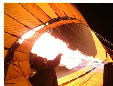
g / A hot air balloon is inflated. Because of thermal expansion, the hot air is less dense than the surrounding cold air, and therefore floats as the cold air drops underneath it and pushes it up out of the way.
