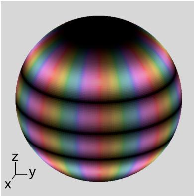
c / A wavefunction on the sphere with |\mathbf{L}| = 11\hbar and L_z = 8\hbar , shown using the color conventions defined in figure u, p. 912.
