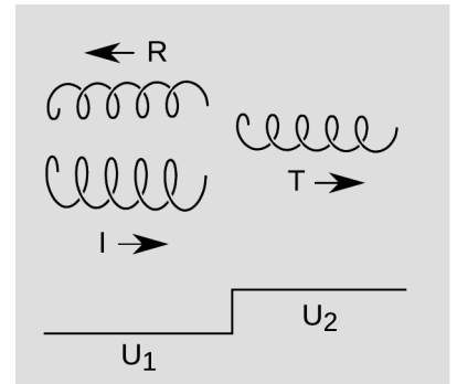
a / An incident wave is partially reflected and partially transmitted at a step in the potential U . The complex wavefunctions are represented using a complex plane perpendicular to the direction of propagation, so that they look like corkscrews. The incident and reflected wavefunctions actually superposed, but are drawn as separate entities and offset for purposes of visualization.
