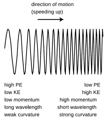
j / An electron in a gentle electric field gradually shortens its wavelength as it gains energy. (As discussed on p. 892, it is actually not quite correct to graph the wavefunction of an electron as a real number unless it is a standing wave, which isn't the case here.)
