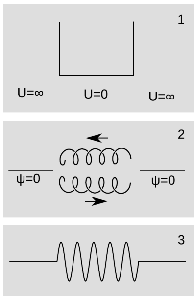
b / A particle in a box.
