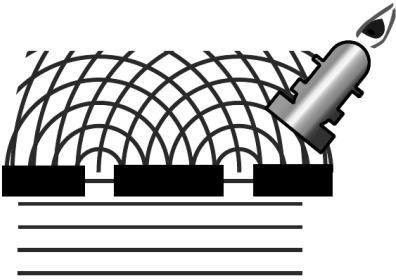
a / Spying on one slit in the double-slit experiment.
