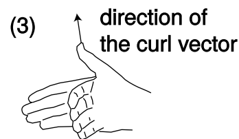
a / The div-meter, 1, and the curl-meter, 2 and 3.
