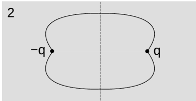
e / The method of images.
