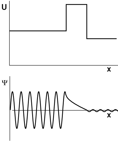
m / Tunneling through a barrier. (As discussed on p. 892, it is actually not quite correct to graph the wavefunction of an electron as a real number unless it is a standing wave, which isn't the case here.)
