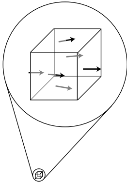
f / The flux through a tiny cube due to a point charge.
