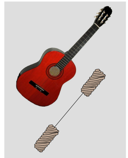
l / We model a guitar string attached to the guitar's body at both ends as a light-weight string attached to extremely heavy strings at its ends.
