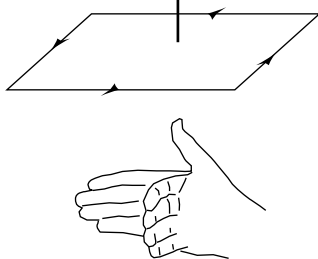
h / The \mathbf{m} and \mathbf{A} vectors.
