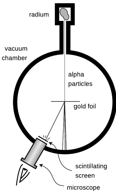
Figure f / Marsden and Rutherford's apparatus.
